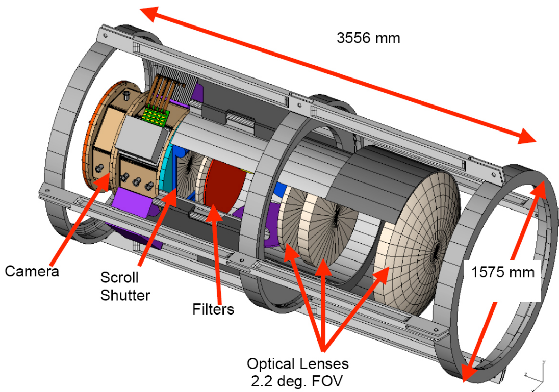
A view of DECam, the camera being built by DES.
