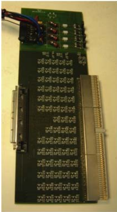
A view of one of the transition boards produced at IFAE.
