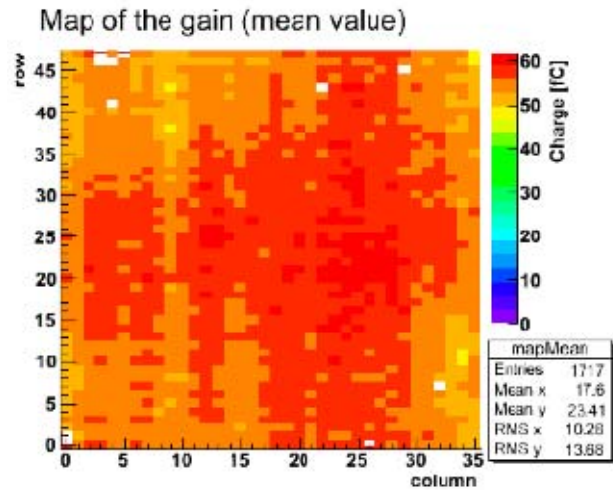
MicroMega gain uniformity obtained with the Test Bench at CERN. The observed non-uniformity is of the order of 10% and it is explained from the capacitance of the readout lines.
