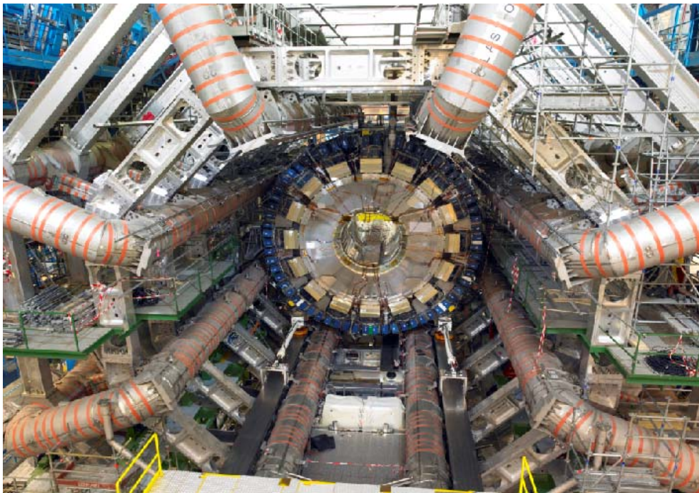
View of the barrel calorimeter in its final position, and the barrel toroid magnets.
