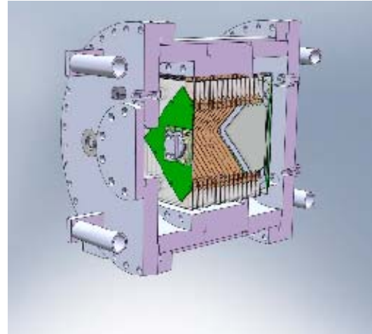
TPC prototype designed at IFAE for test of readout technology for the NEXT project. The TPC will be able to hold 10 atm.
