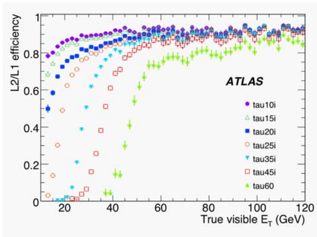
Efficiency curves of Level-2 tau selection relative to Level-1 for different tau energy thresholds.
