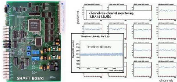
Top layer of the 6-layers SHAFT board, designed and built at IFAE (left), and example of monitoring of the stability of the PMTs of one of Tilecal module.
