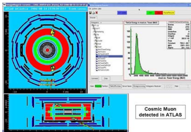
ATLAS Event Display showing a cosmic ray going through the detector (left) and energy deposited by cosmic muons in the Tilecal calorimeter (right)
