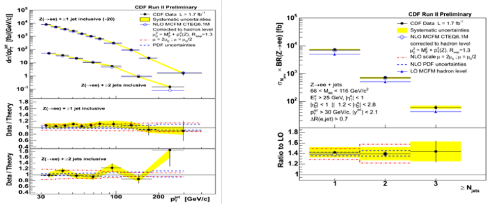
Figure: Measured Z + jets Cross Sections compared to pQCD NLO prediction.
