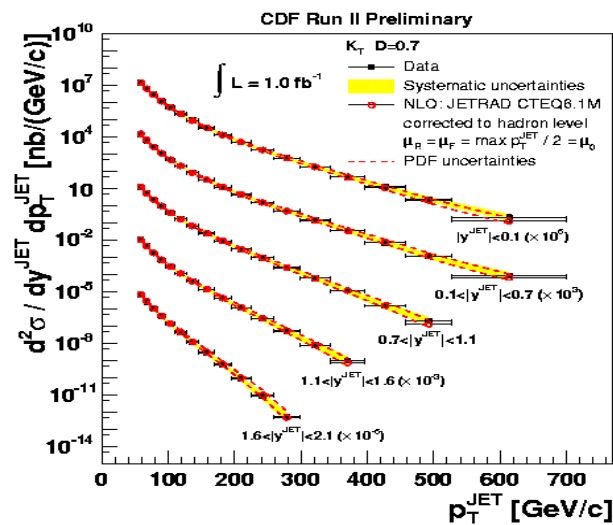
Measured inclusive jet cross section using the K_T algorithm.
