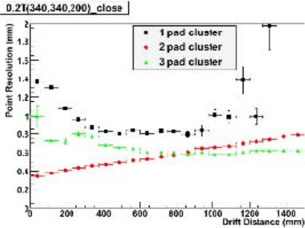
Point resolution obtained with a MicroMega prototypes at CERN. The resolution is shown for clusters with one two or three readout channels.
