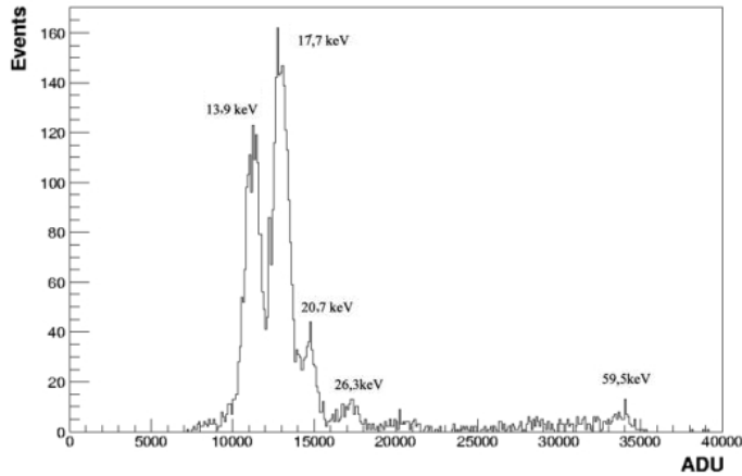
Left: Americium 241 spectrum showing the characteristic peaks measured with a test CCD in the test set-up at IFAE. Right: Expected spectrum. The leftmost peak lies inside the pedestal region of the set-up, and, hence, could not be measured.
