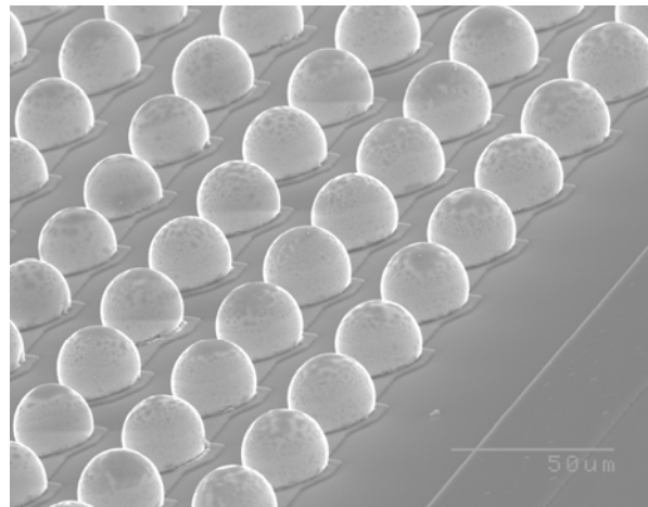
An array of solder bumps with 50\mu\text{m} pitch developed by CNM to be used with the FC150 machine.
