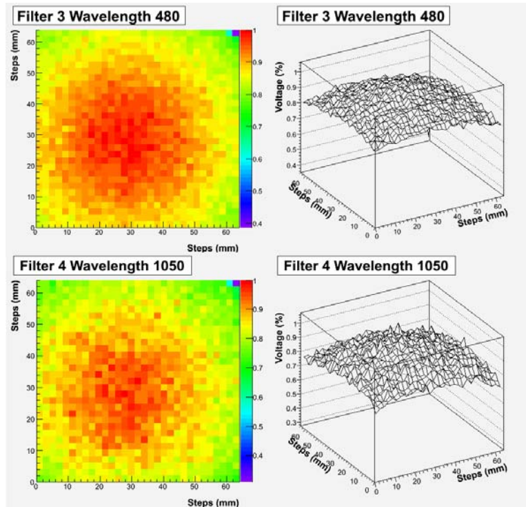
Transmission maps for the whole CCD test set-up, for two different wavelengths, 480 nm (top), 1050 nm (bottom). Maps like these were obtained for wavelengths between 300 nm and 1200 nm at 5 nm intervals.
