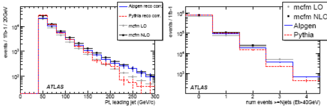
Unfolded transverse energy of the leading jet (left) and number of expected events at hadron level (right) in Pythia and Alpgen Z(\rightarrow\mu^+\mu^-) + jets Monte Carlo, shown along with predictions from MCFM for an integrated luminosity of 1 \text{ fb}^{-1} .
