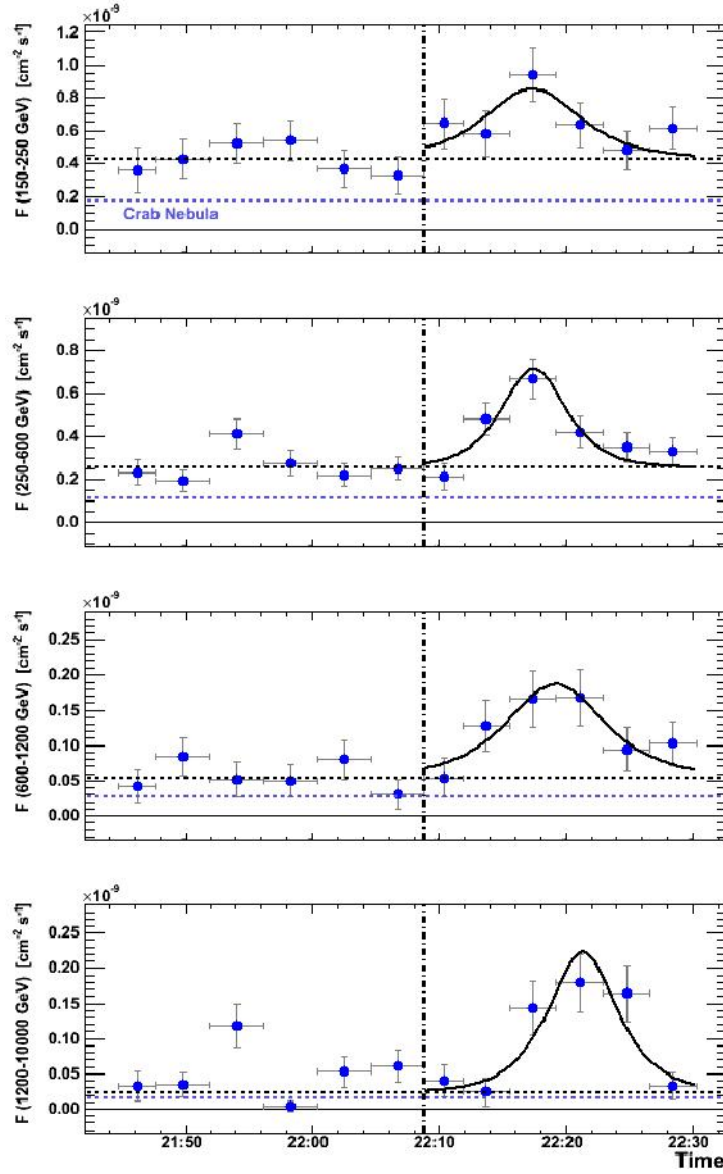
A short-lasting episode (flare) of gamma ray emission in the AGN Markarian 501. The flare is the shortest ever observed in gamma rays. The figure shows the gamma ray flux as a function of time for four different energy bands, ranging from 150-250 GeV at the top panel to >1200 GeV at the bottom. The flare arrives later with growing energy.
