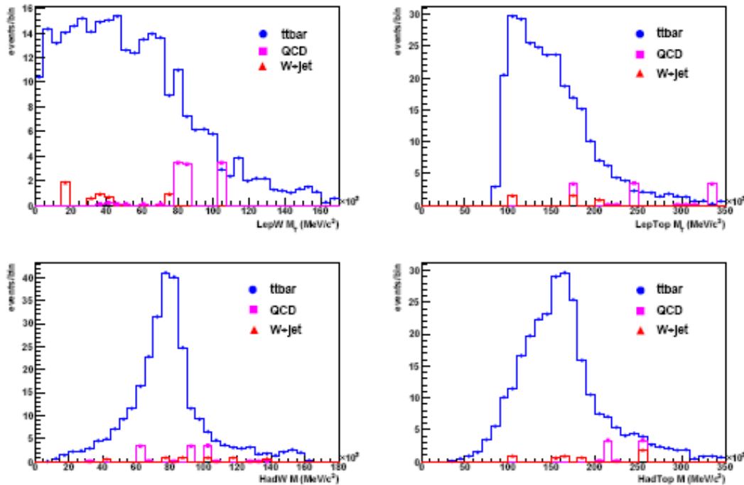
Top: leptonic W (left) and top (right) transverse masses. Bottom: hadronic W (left) and top (right) invariant masses. The plots correspond to an integrated luminosity of 100 \text{ pb}^{-1} . Signal is shown in circles, QCD background with squares and W+jets background with triangles.
