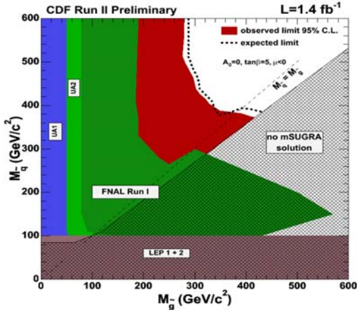
Squark/Gluino exclusion plane. The red band indicates the results from this analysis.
