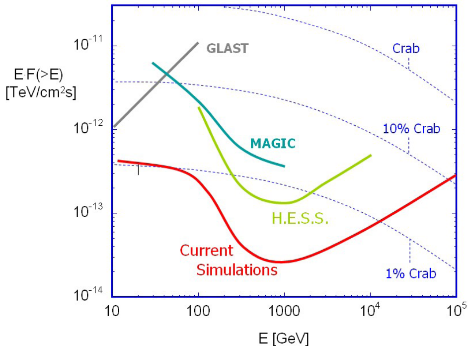
Expected sensitivity of CTA compared with the sensitivity of the best current installations.
