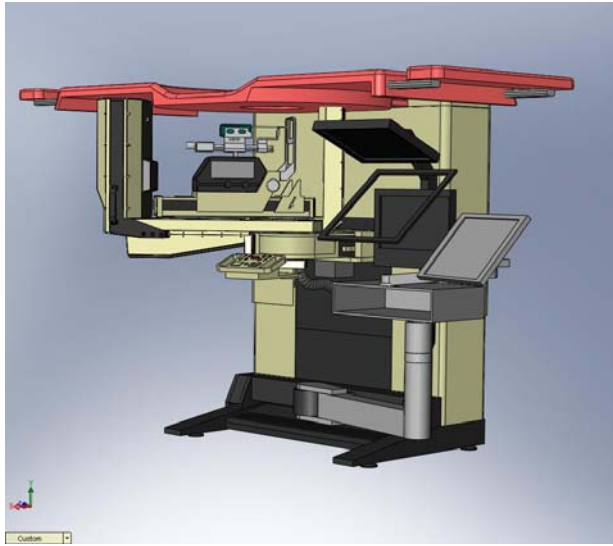
CAD presentation of the 3D breast biopsy machine which will be commissioned in early 2008
