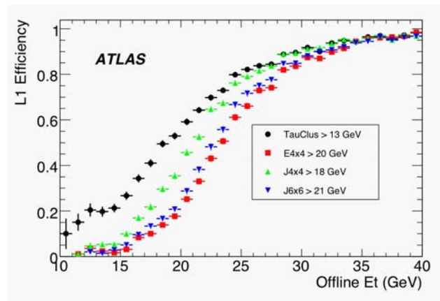
Trigger efficiency curves for different Level-1 energy reconstruction methods as a function of the offline transverse energy.
