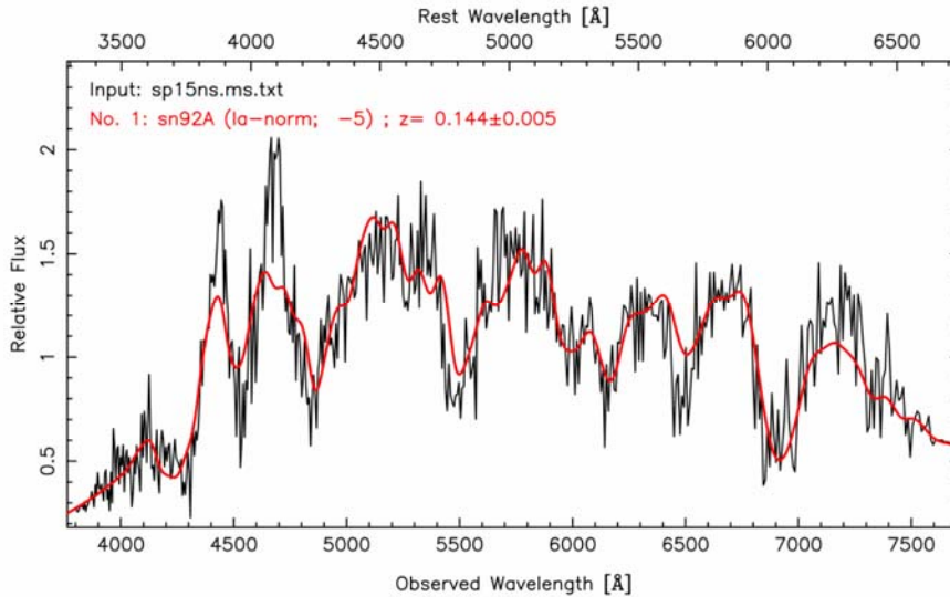
Spectrum of supernova SN2007ph, at redshift z=0.144 , taken on November 5 th 2007 at TNG. Superimposed is a template of a standard type-Ia supernova redshifted to z=0.144 , observed five days before maximum light.
