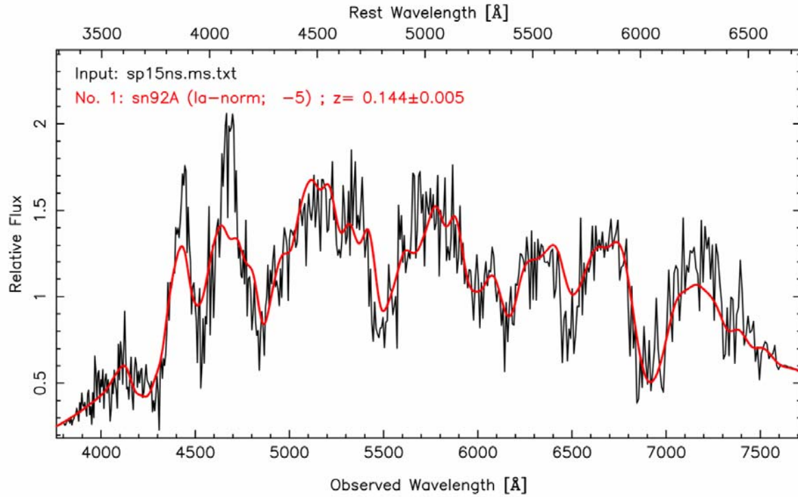
Spectrum of supernova SN2007ph, at redshift z=0.144 , taken on November 4 th 2007 at TNG. The lower scale shows wavelengths in the observer frame, while the top scale shows the same wavelengths in the supernova frame. The characteristic broad Si-II feature at about 6000 Angstrom in the supernova frame is clearly visible. Superimposed is a template of a standard type-Ia supernova redshifted to z=0.144 , observed 5 days before maximum light. The match between the two spectra is excellent.
